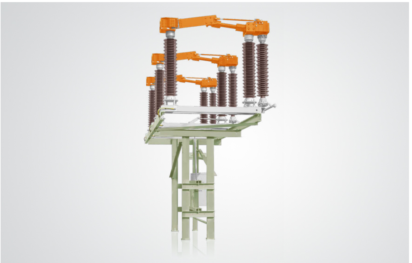
Vertical Disconnecter 123 kV
